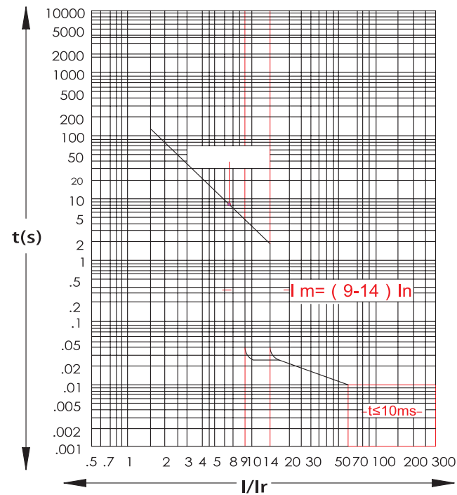
MNX400/630 - TMM
