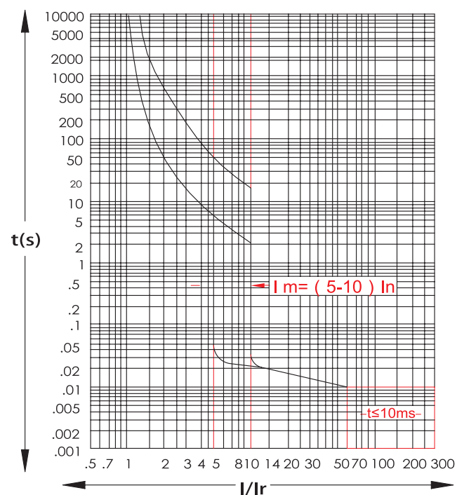
MNX400/630 - TMD
