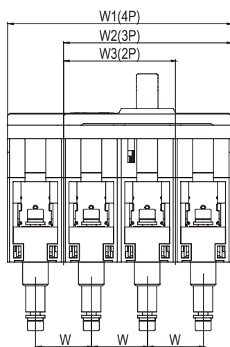
MNX125/160/250
