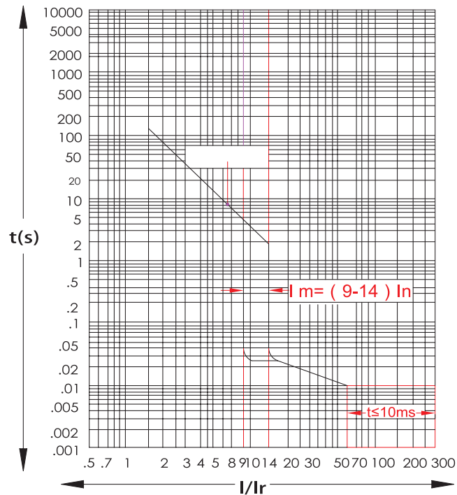
MNX125 - TMM
