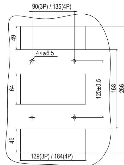
MNX400/630
