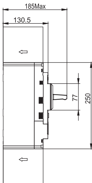
MNX400/630V
