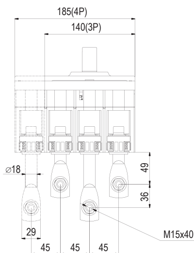
MNX400/630
