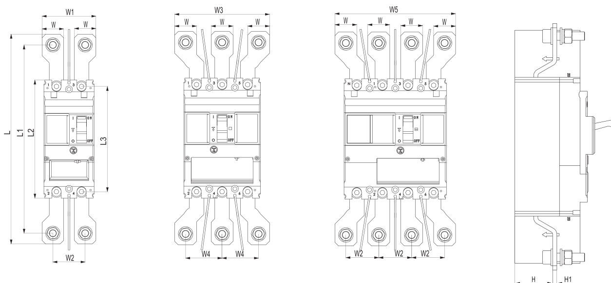
MNX125/160/250/400/630
